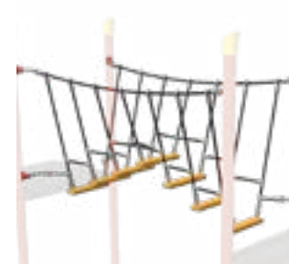
Catwalk Net Bridge Ages: 5-12 Decks: Equal Height Up to 4' Length: 8' Black Netting Only
